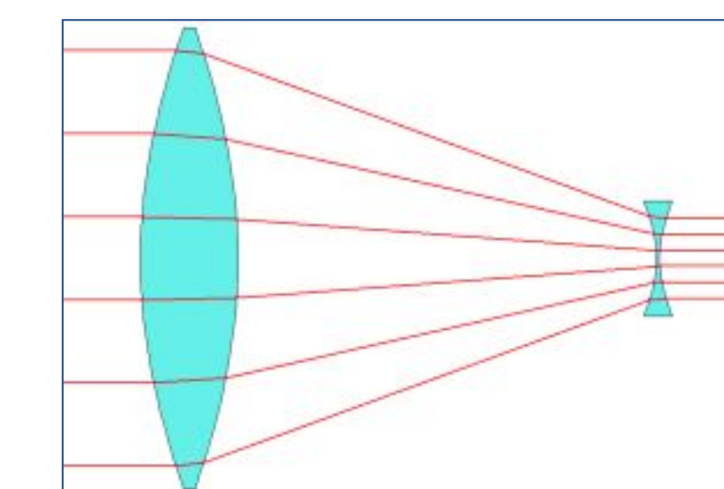
Galilean System: optical magnifying system
