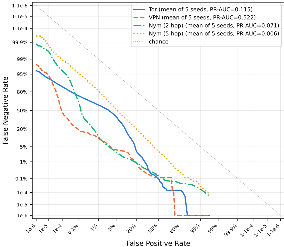
DET curves: pointwise mean of 5 seeds per mode
