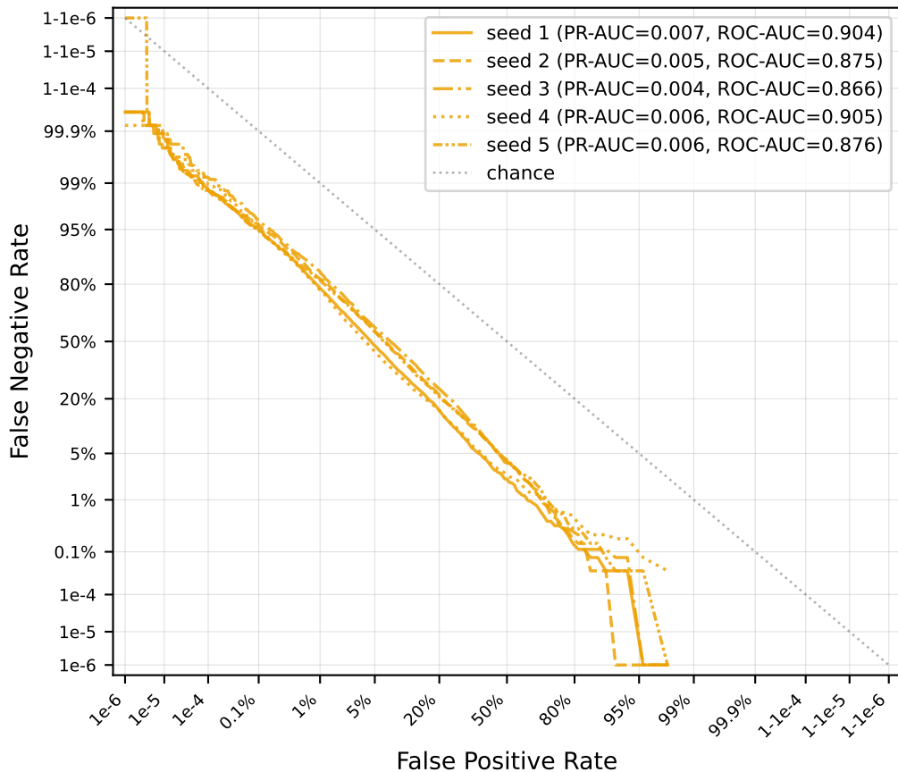
DET curves, all 5 seeds: Nym (5-hop)
