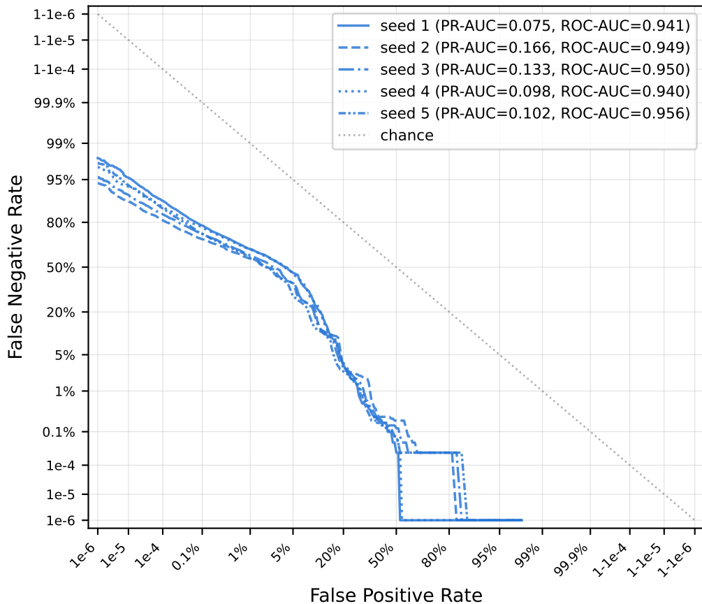
DET curves, all 5 seeds: Tor
