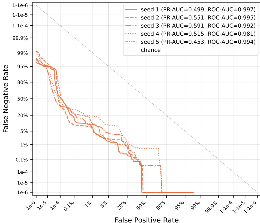
DET curves, all 5 seeds: VPN
