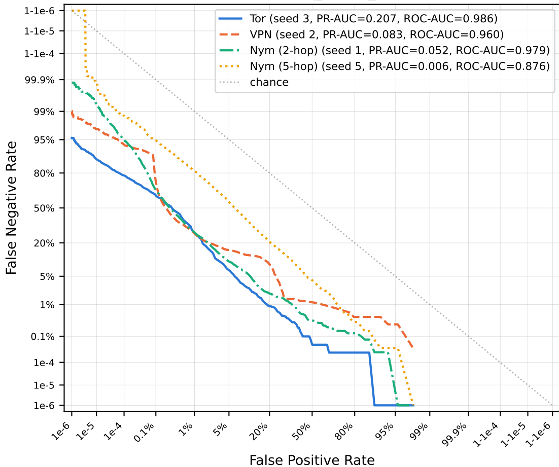
DET curves: one representative run per mode (curve shape only -- see cross_mode_mean.pdf for ranking)
