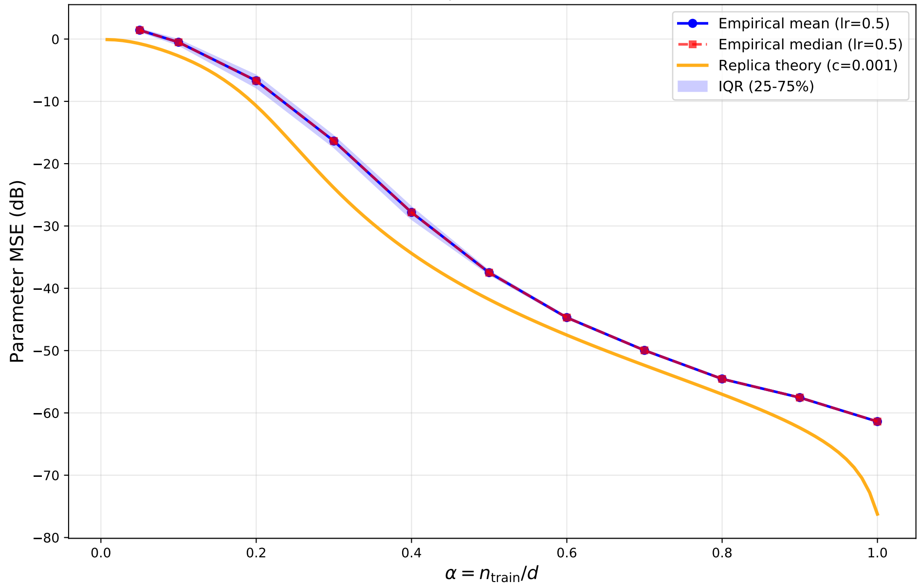
Empirical vs Replica Theory ( \text{lr}=0.5 , c=0.001 ) Bernoulli-Gaussian, \rho = 0.040 , successes = 14/22
