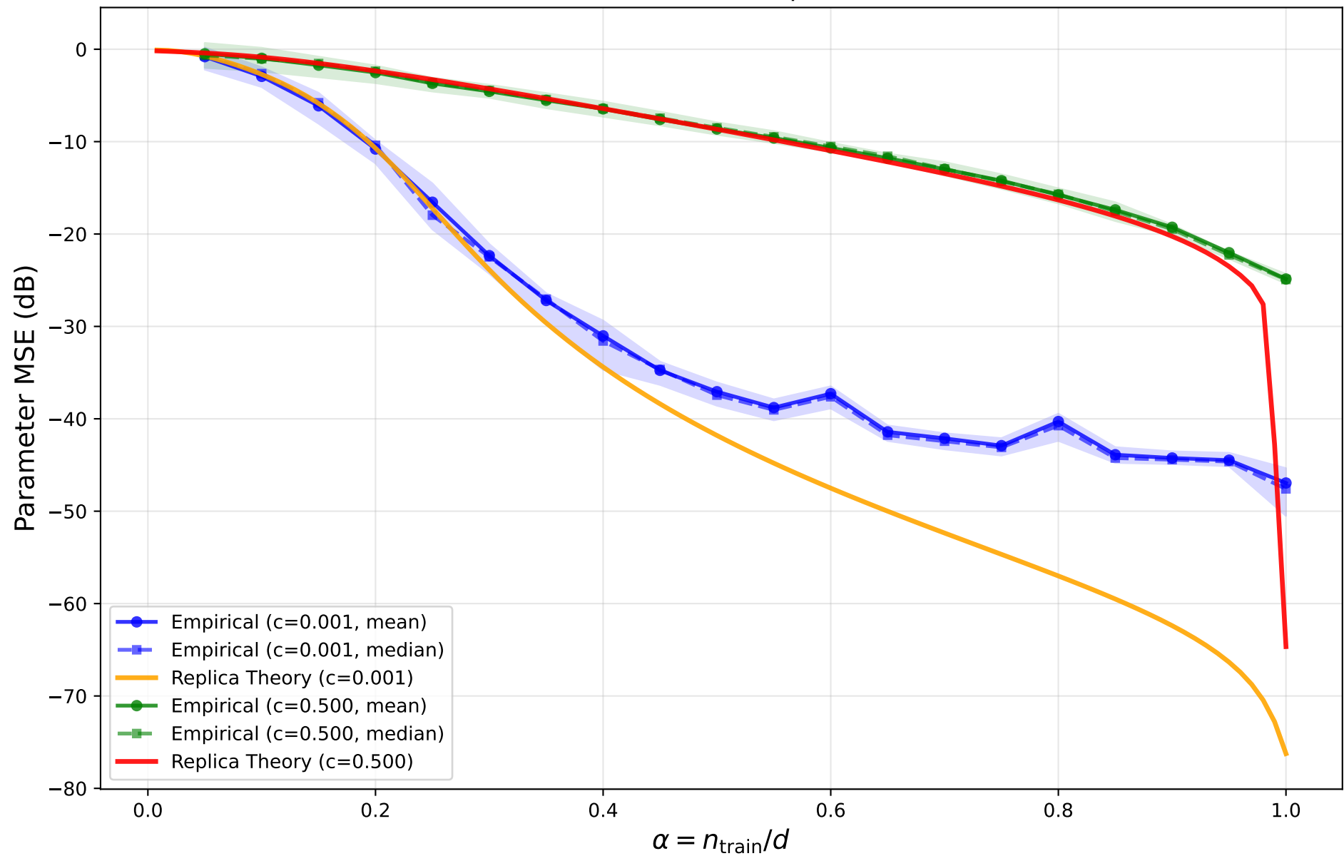
Generalization Curves: Empirical vs Replica Theory Bernoulli-Gaussian, \rho = 0.040
