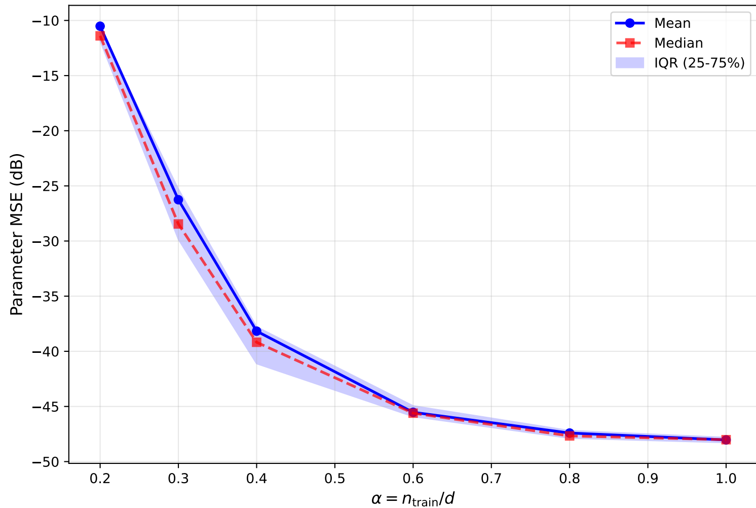
Generalization Curve (Bernoulli-Gaussian, \rho = 0.040 , c = 0.000 ) successes = 0 / 60
