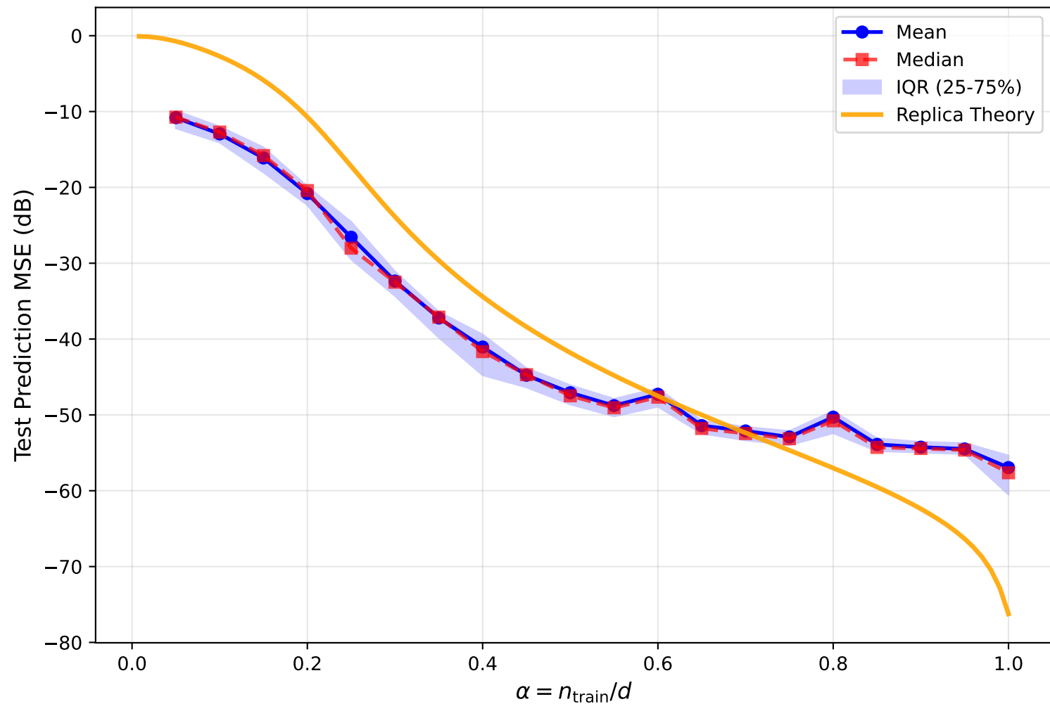
Generalization Curve (Bernoulli-Gaussian, \rho = 0.040 , c = 0.001 ) successes = 13 / 120
