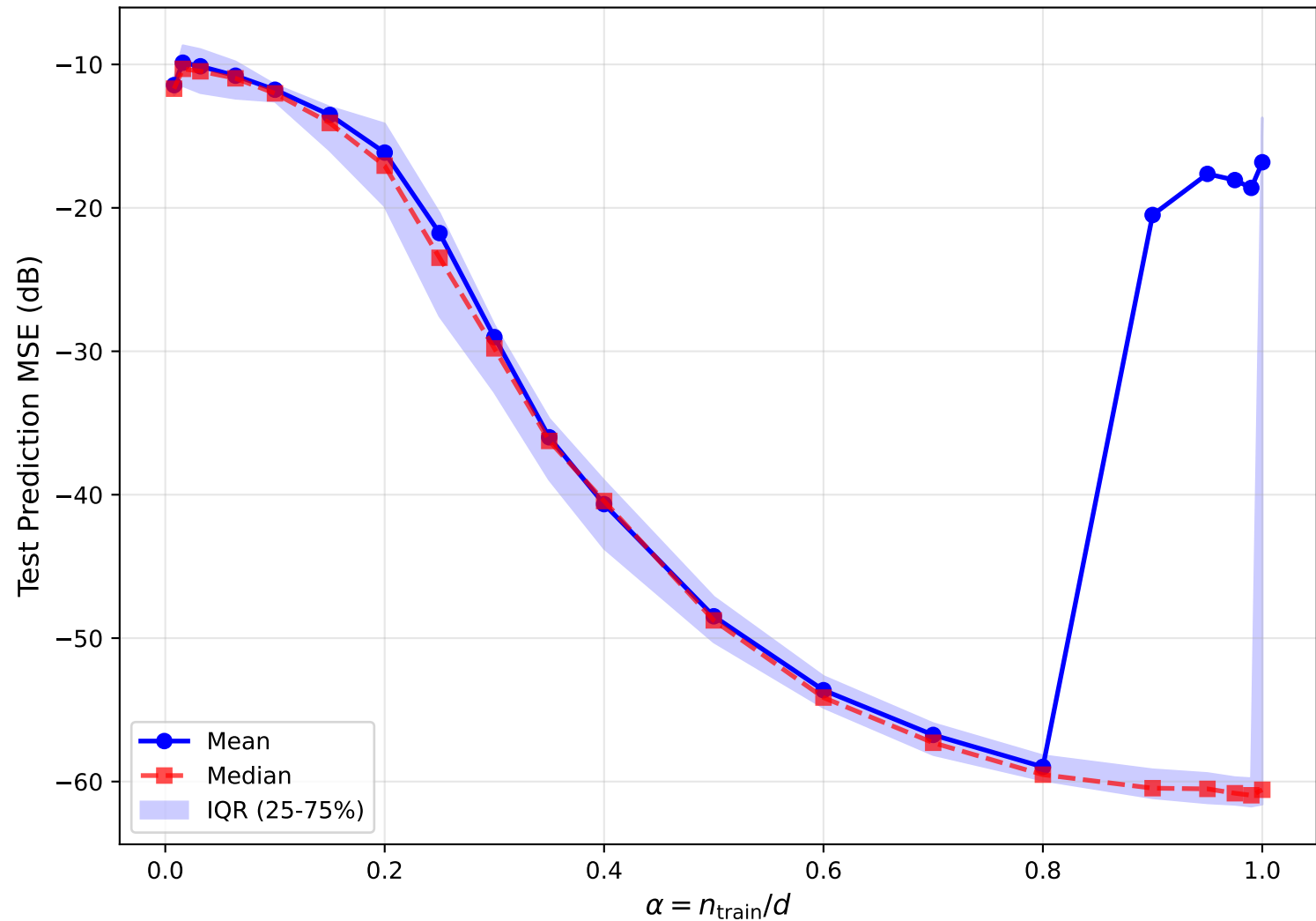
Generalization Curve (Bernoulli-Gaussian, \rho = 0.040 )
