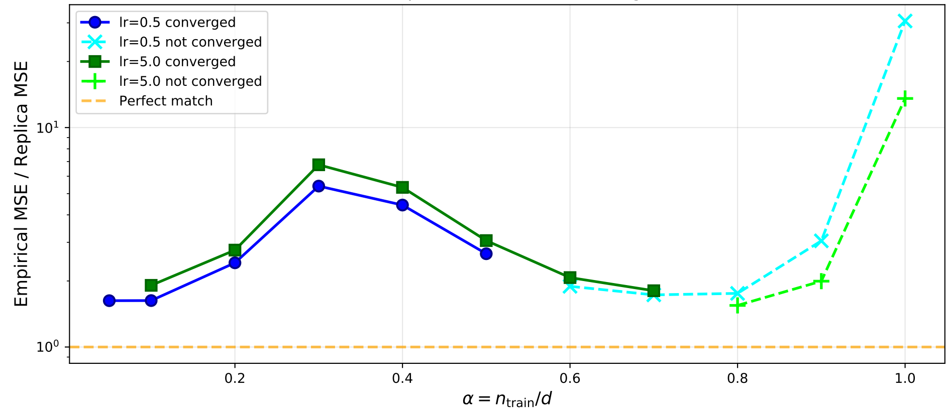
Ratio Comparison: Different Learning Rates
