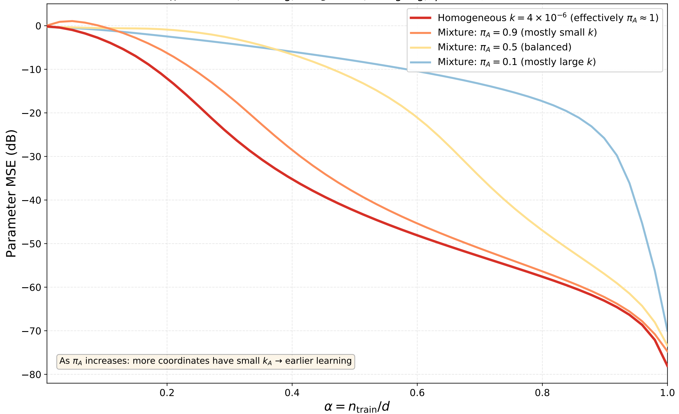
Mixture Mode Interpolation: Varying \pi_A k_A = 4e - 06 (weak reg) vs k_B = 1.0 (strong reg), \rho = 0.04 , \lambda = 1e - 06
