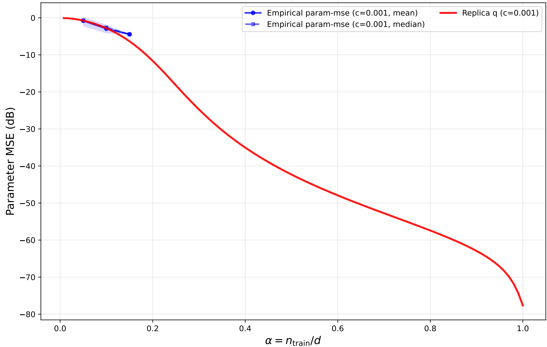
Generalization Curves: Empirical vs Replica Theory Bernoulli-Gaussian ( \rho = 0.040 ), Noiseless
