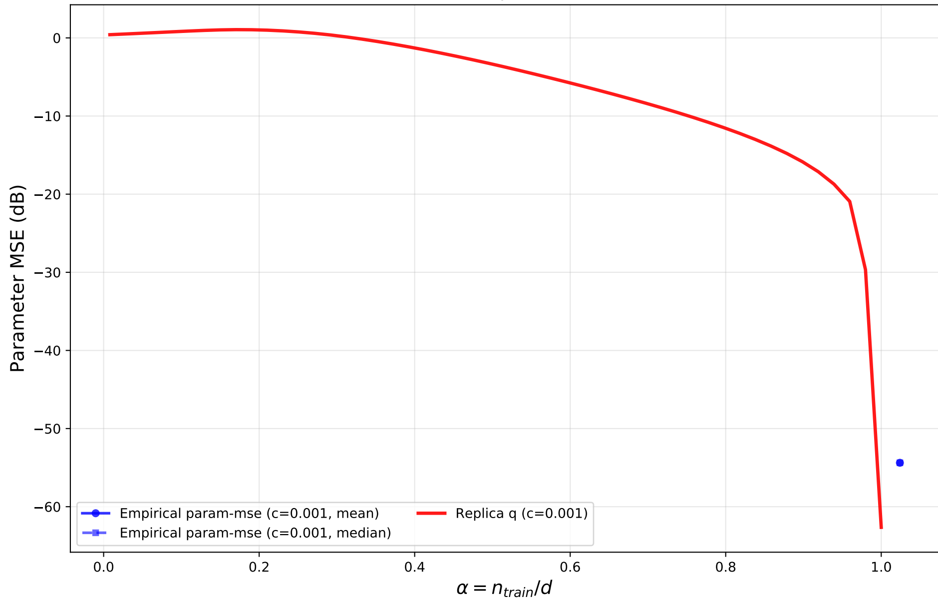
Generalization Curves: Empirical vs Replica Theory Bernoulli-Gaussian ( \rho = 0.010 ), Noiseless
