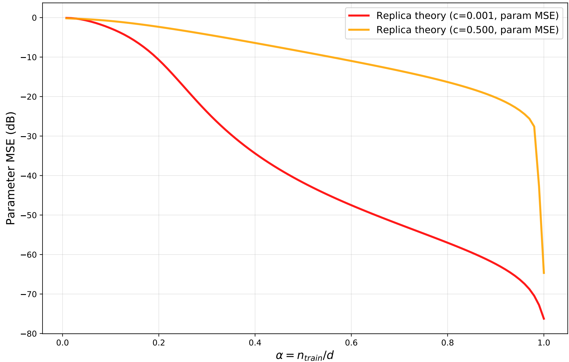
Replica Theory Curves: Parameter MSE Bernoulli-Gaussian ( \rho = 0.040 ), Noiseless, \lambda = 1e - 06
