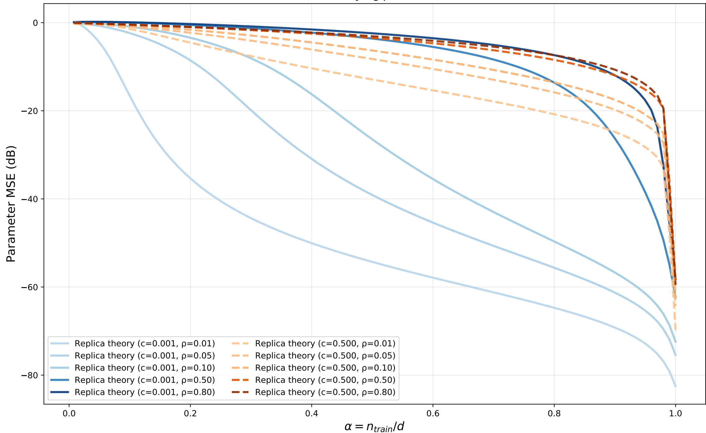
Replica Theory Curves: Parameter MSE Bernoulli-Gaussian (varying \rho ), Noiseless, \lambda = 1e - 06
