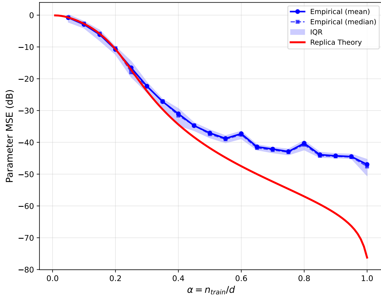
Step 0 Validation: c = 0.001 \rho = 0.04 , Stable: ✓, Match: ✓ ( r=0.972 ), Converged: ✗
