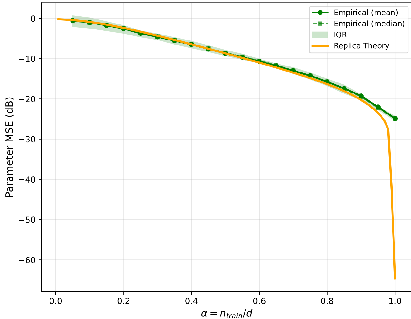
Step 0 Validation: c = 0.5 \rho = 0.04 , Stable: ✓, Match: ✗ ( r=0.845 ), Converged: ✗
