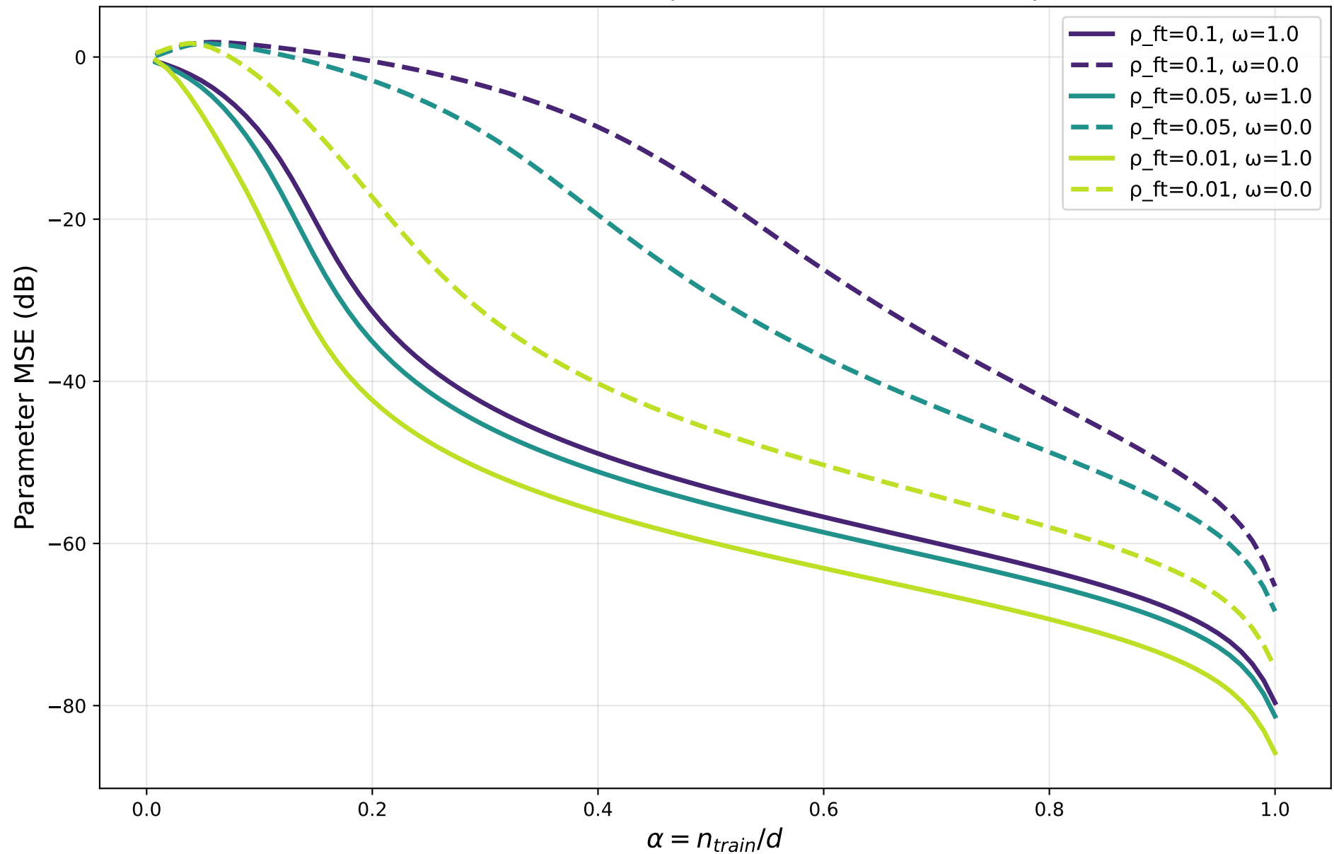
FT Sparsity Comparison ( \rho_{pt}=0.1 fixed) Solid: \omega=1.0 (full overlap), Dashed: \omega=0.0 (no overlap)
