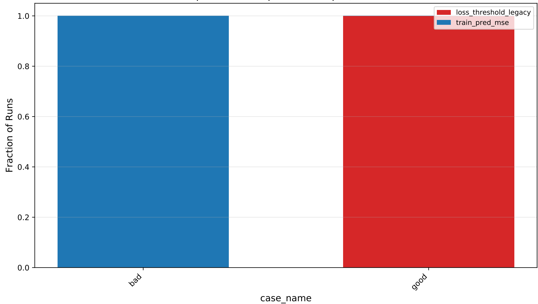
Stop Reason Composition - step2 ( \alpha=0.05 )
