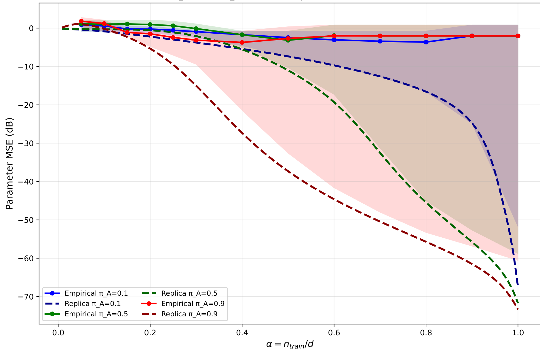
Step 1 Validation: Mixture-k Heterogeneous Init c_A=0.001 , c_B=0.5 , \rho=0.04 | Ordering: \mathbf{X} , Smooth: \mathbf{X}
