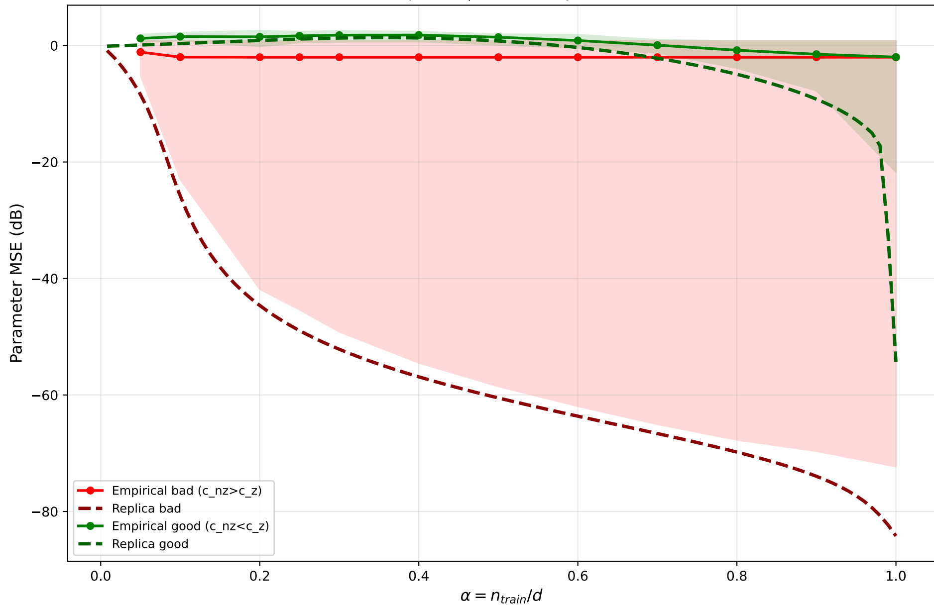
Step 2 Validation: Support-Conditioned k Init \rho=0.04 | Directionality: \times
