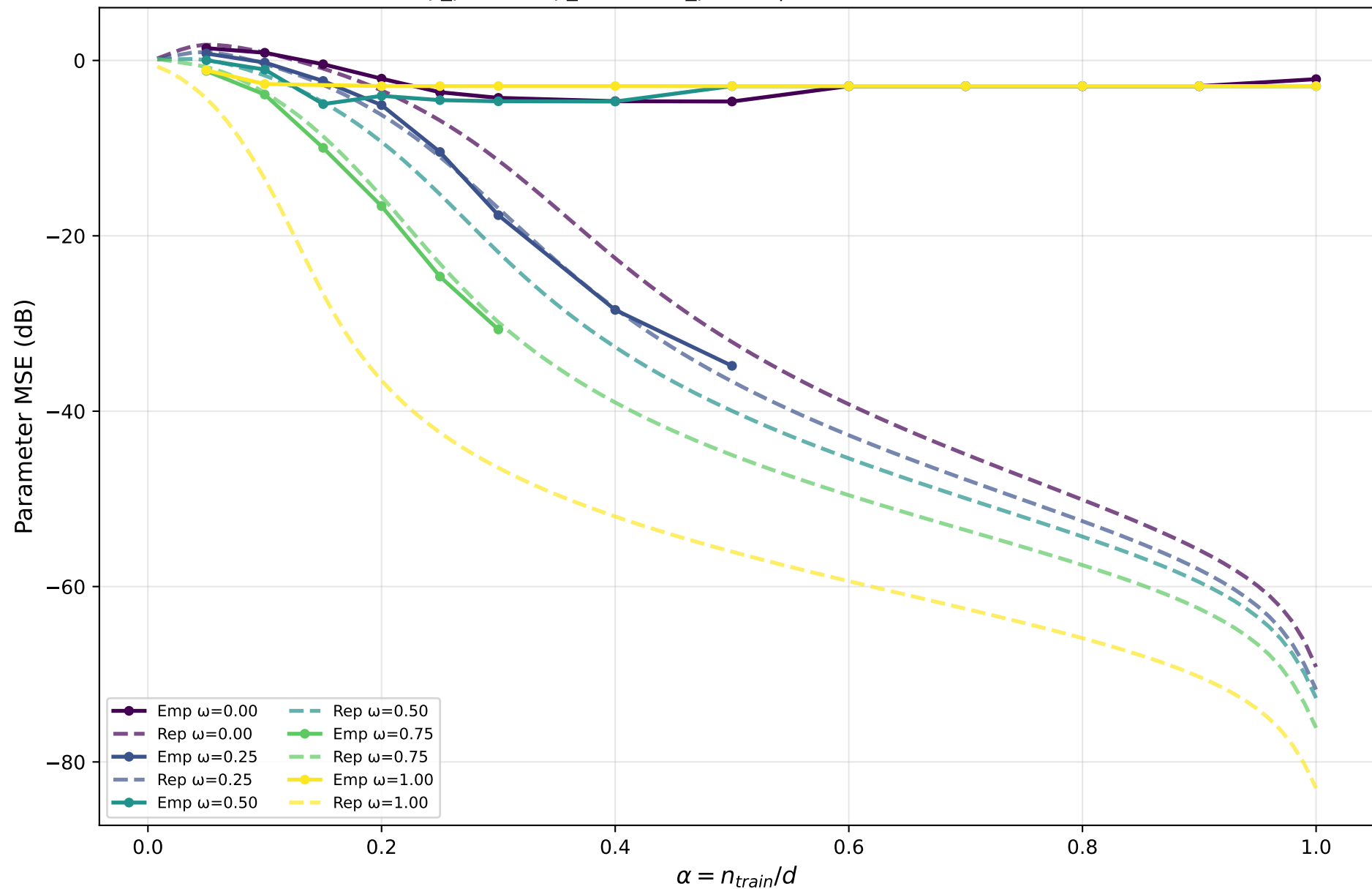
Step 3 Validation: PT+FT Oracle (Omega Sweep) \rho_{pt}=0.10 , \rho_{ft}=0.04 , a_{pt}=1.0 | Monotonic: \times , Match: \times
