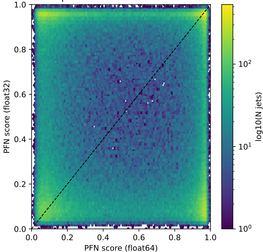
PFN output correlation: float64 vs float32
