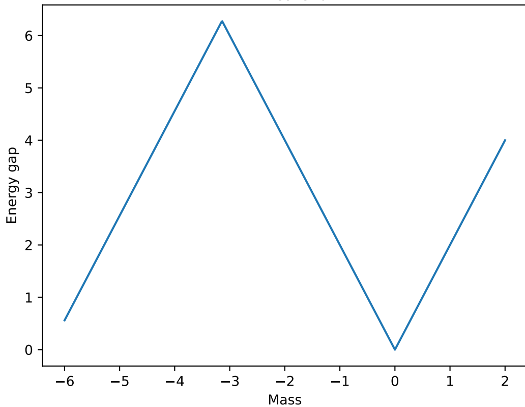
Energy gap
