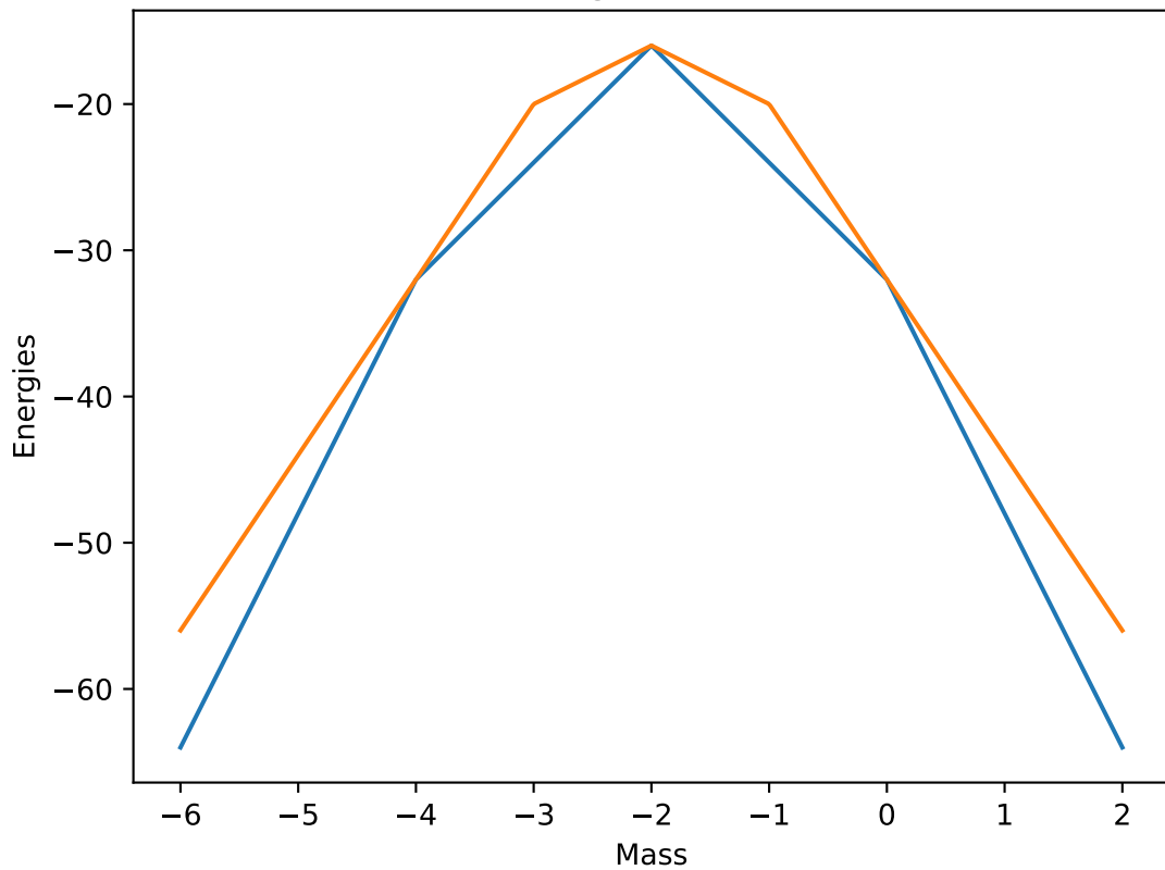
Energies for r=1
