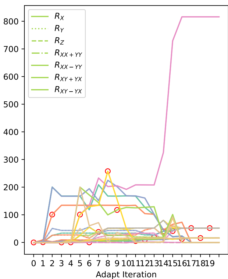
Second derivative
