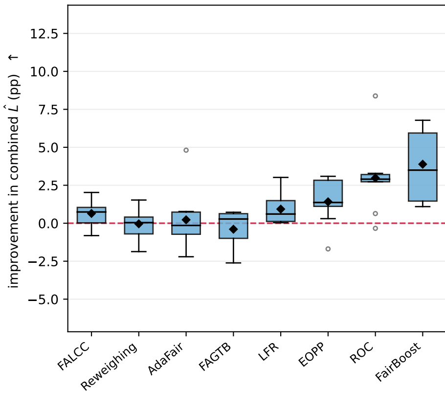
combined \hat{L}
