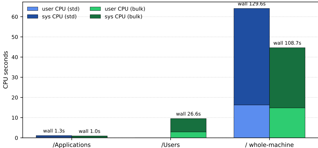
CPU time: std lstat vs getattrlistbulk
