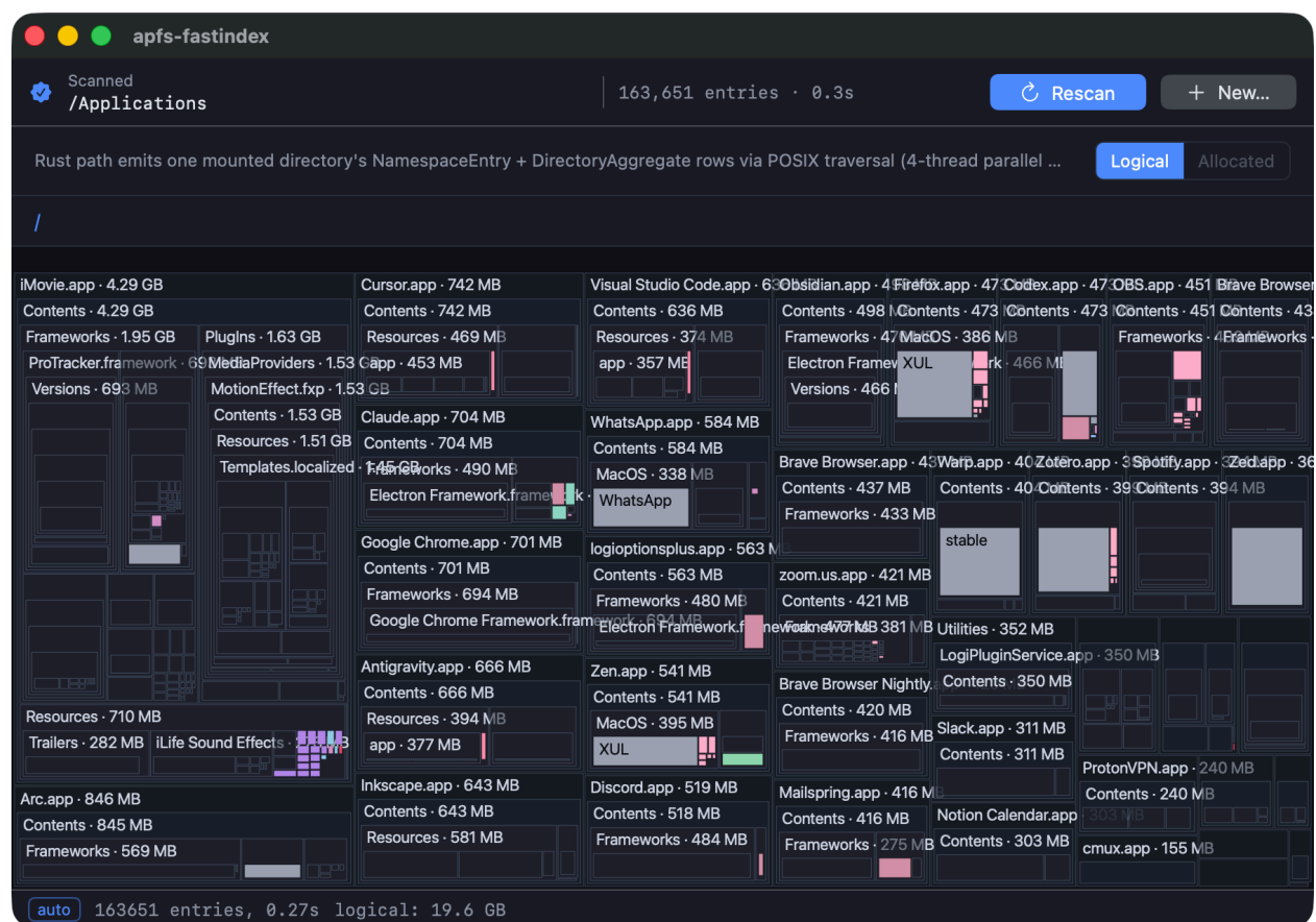
Figure 13.3: A loaded scan of /Applications : 163,651 entries in 0.3 s (the four-thread parallel fallback). Leaf rectangles carry path and size; the colour family encodes file kind. The status bar reads the total logical bytes for the visible aggregate.
