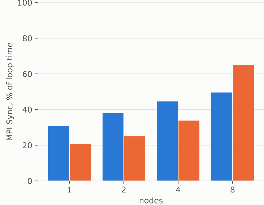
Time spent waiting for other ranks
