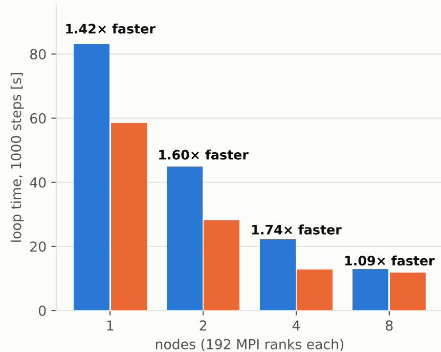
Time to run 1000 steps
