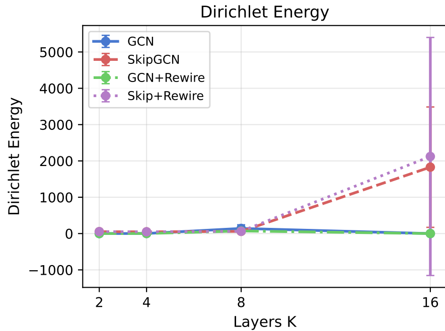
Experiment A: Oversmoothing - SBM graph (mean \pm std over 5 seeds)
