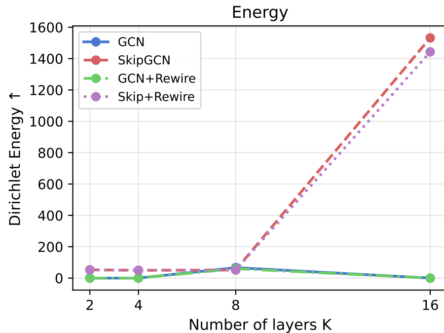
Experiment A: Oversmoothing on SBM graph
