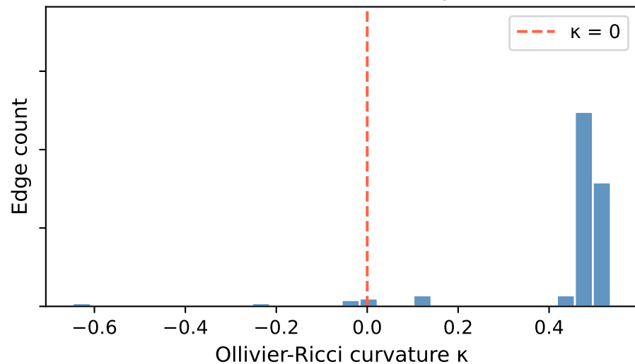
After SDRF rewiring
