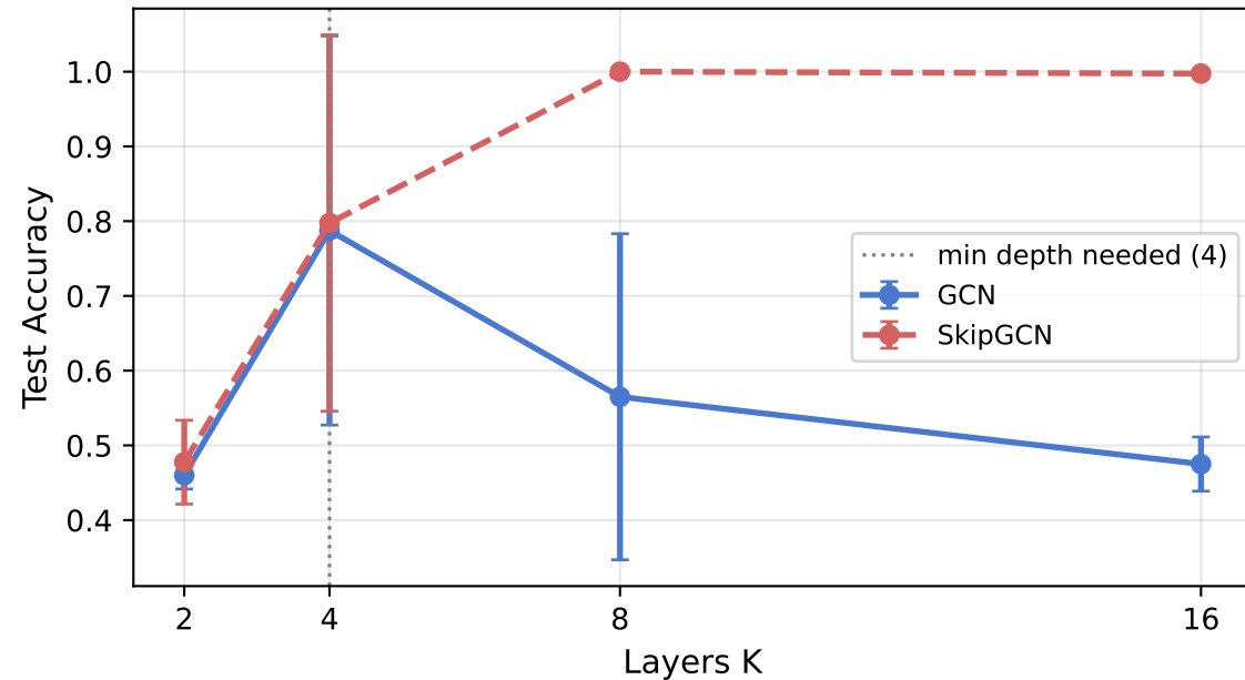
Acc vs Depth (bridge_length=3)
