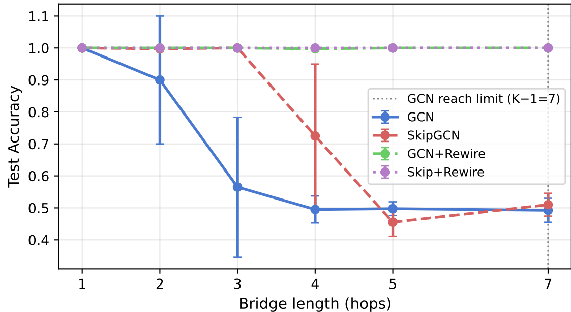
Acc vs Bridge Length (K=8)
