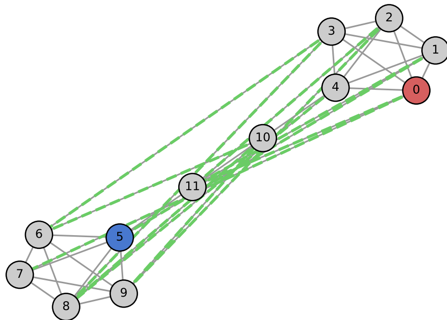
After SDRF rewiring
