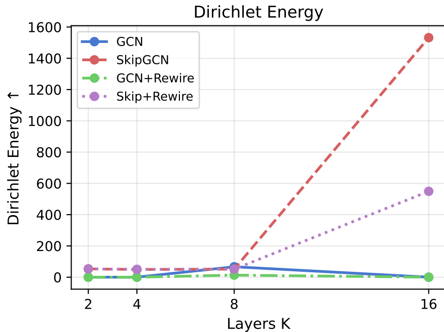
Experiment A: Oversmoothing — SBM graph
