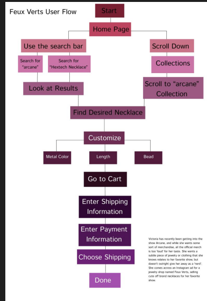
User Flow
