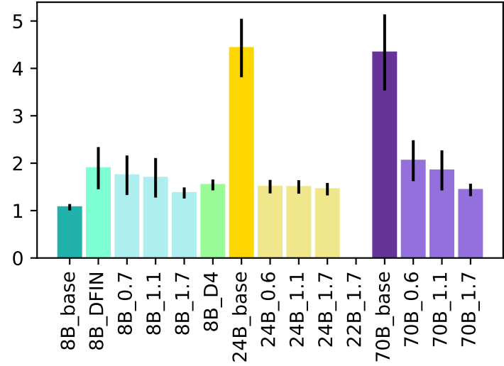
Average Changed Cell Count
