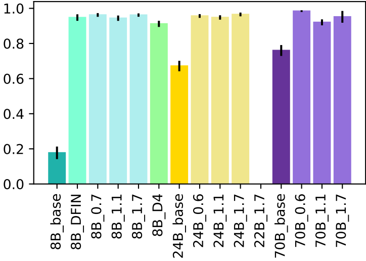
Truncated Kappa
