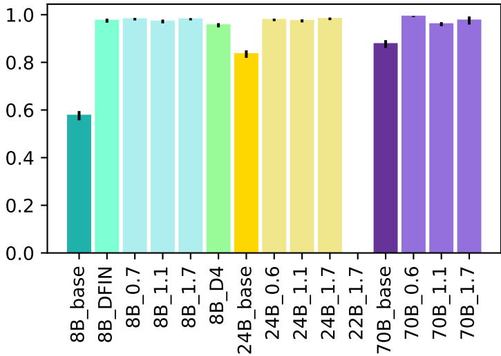
Accuracy
