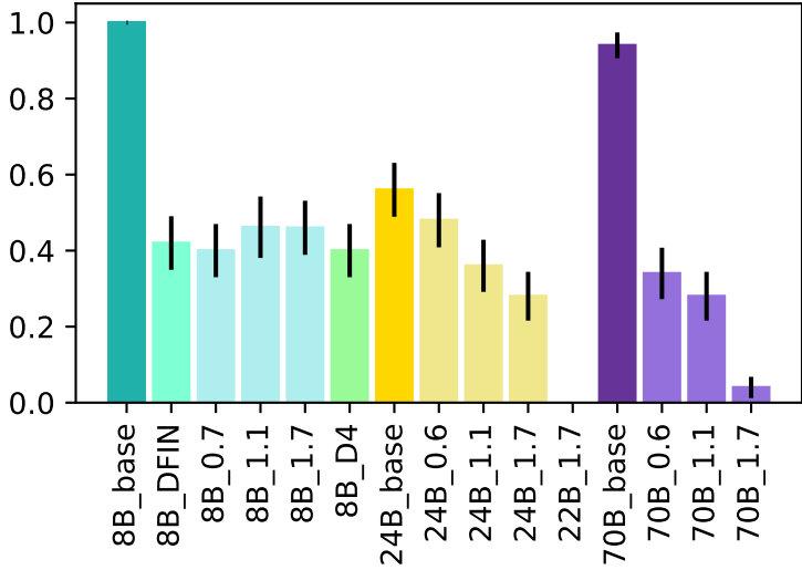
Lose
