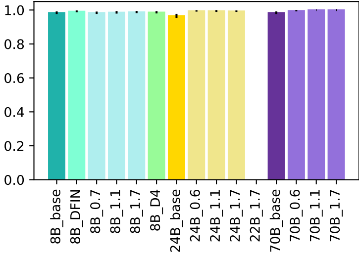
Slot-Filling-Accuracy
