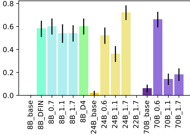
Success
