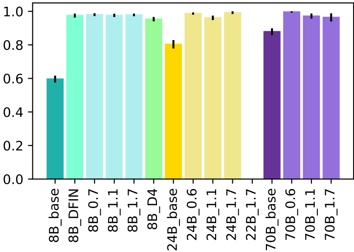
Middle-Accuracy
