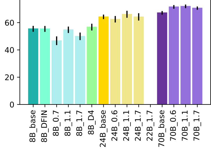
Main Score
