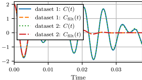
Real part dipole correlation
