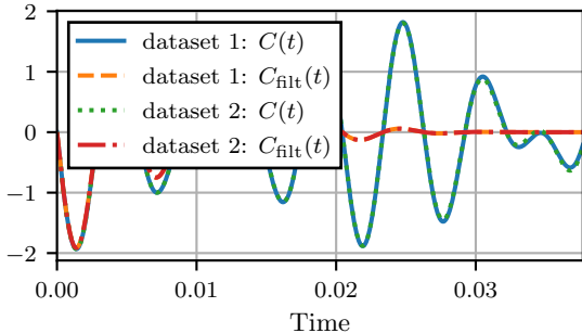
Imaginary part dipole correlation
