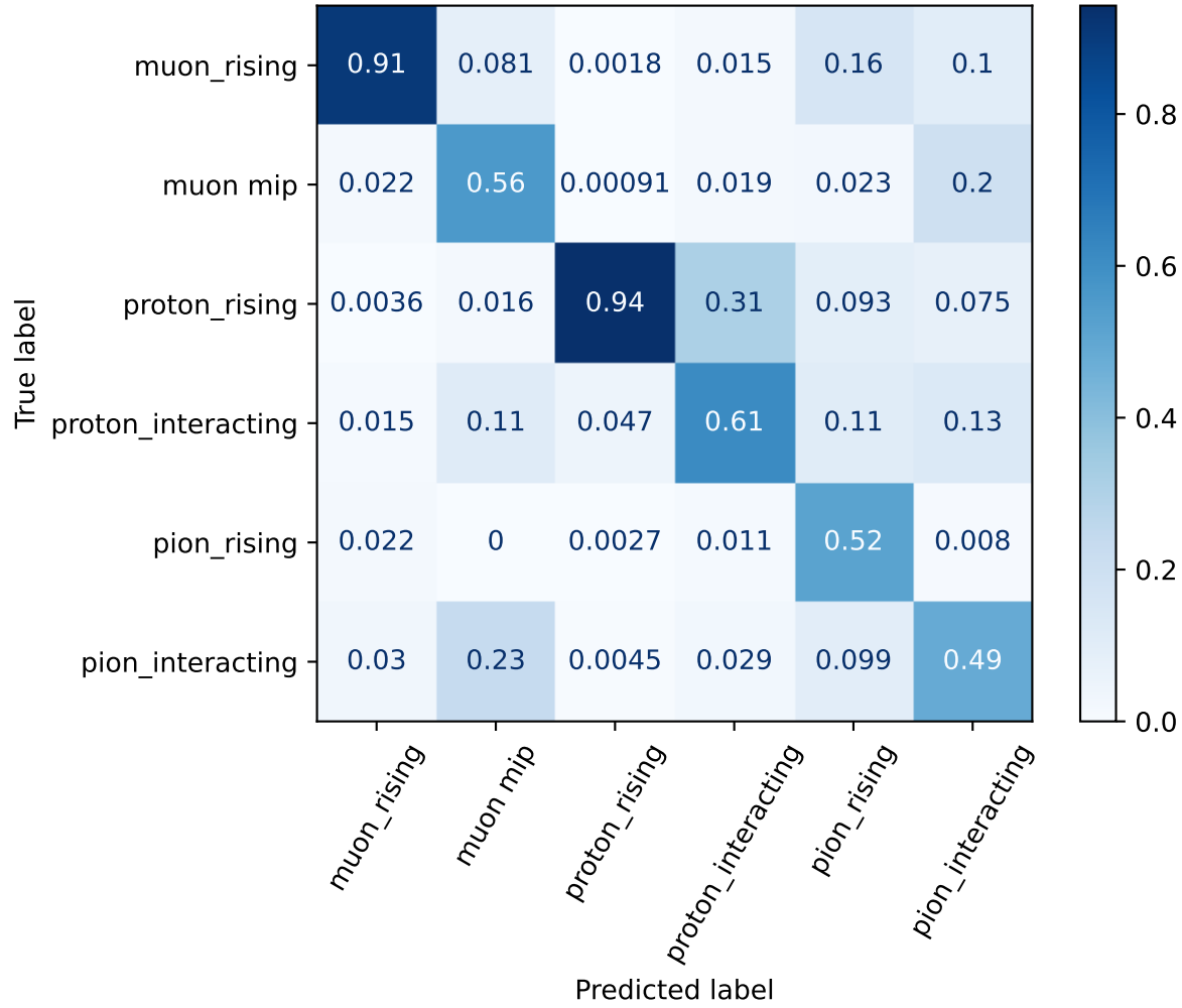
purity confusion matrix - learning rate: 0.01 max depth: 5 subsample frac: 0.4
