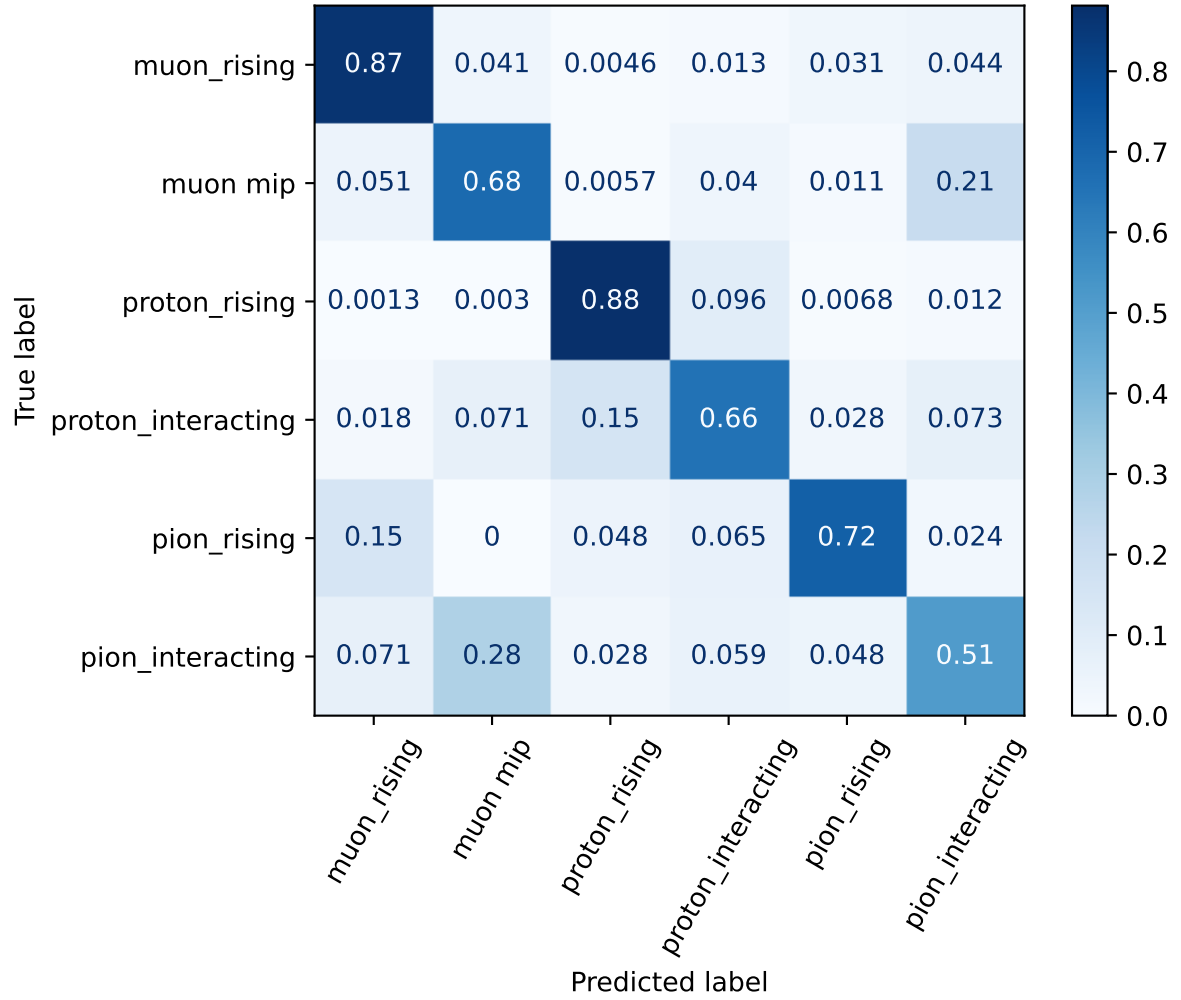
efficiency confusion matrix - learning rate: 0.01 max depth: 5 subsample frac: 0.4
