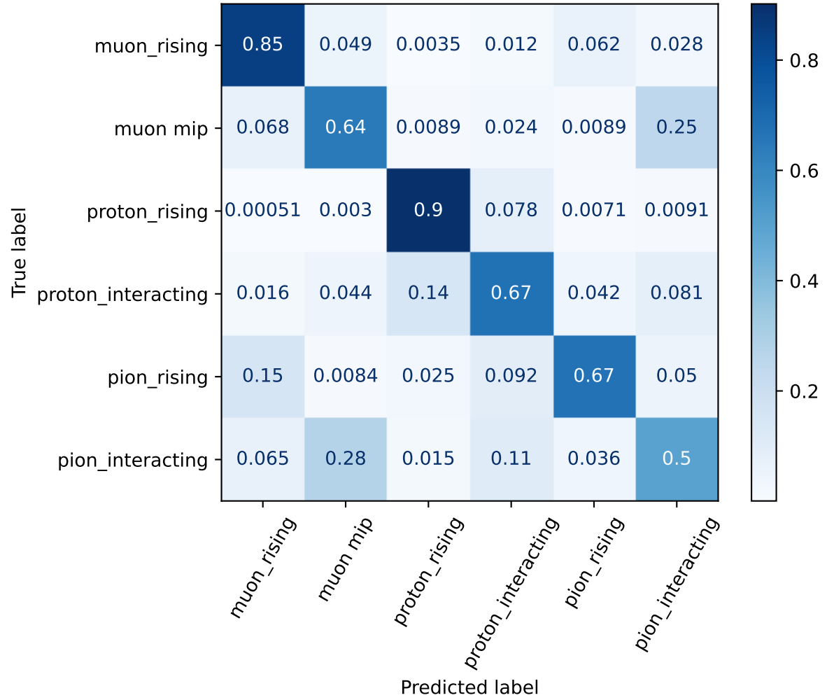
efficiency confusion matrix - learning rate: 0.025 max depth: 5 subsample frac: 0.4
