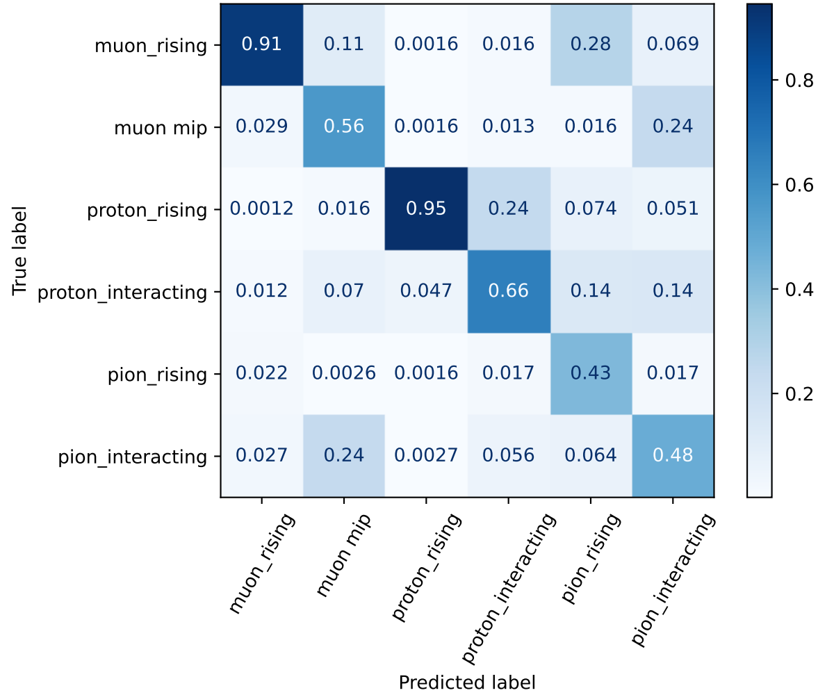
purity confusion matrix - learning rate: 0.025 max depth: 5 subsample frac: 0.4
