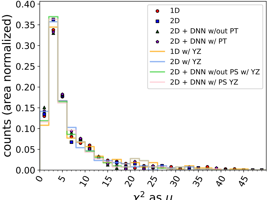
MUONS \chi^2 as \mu
