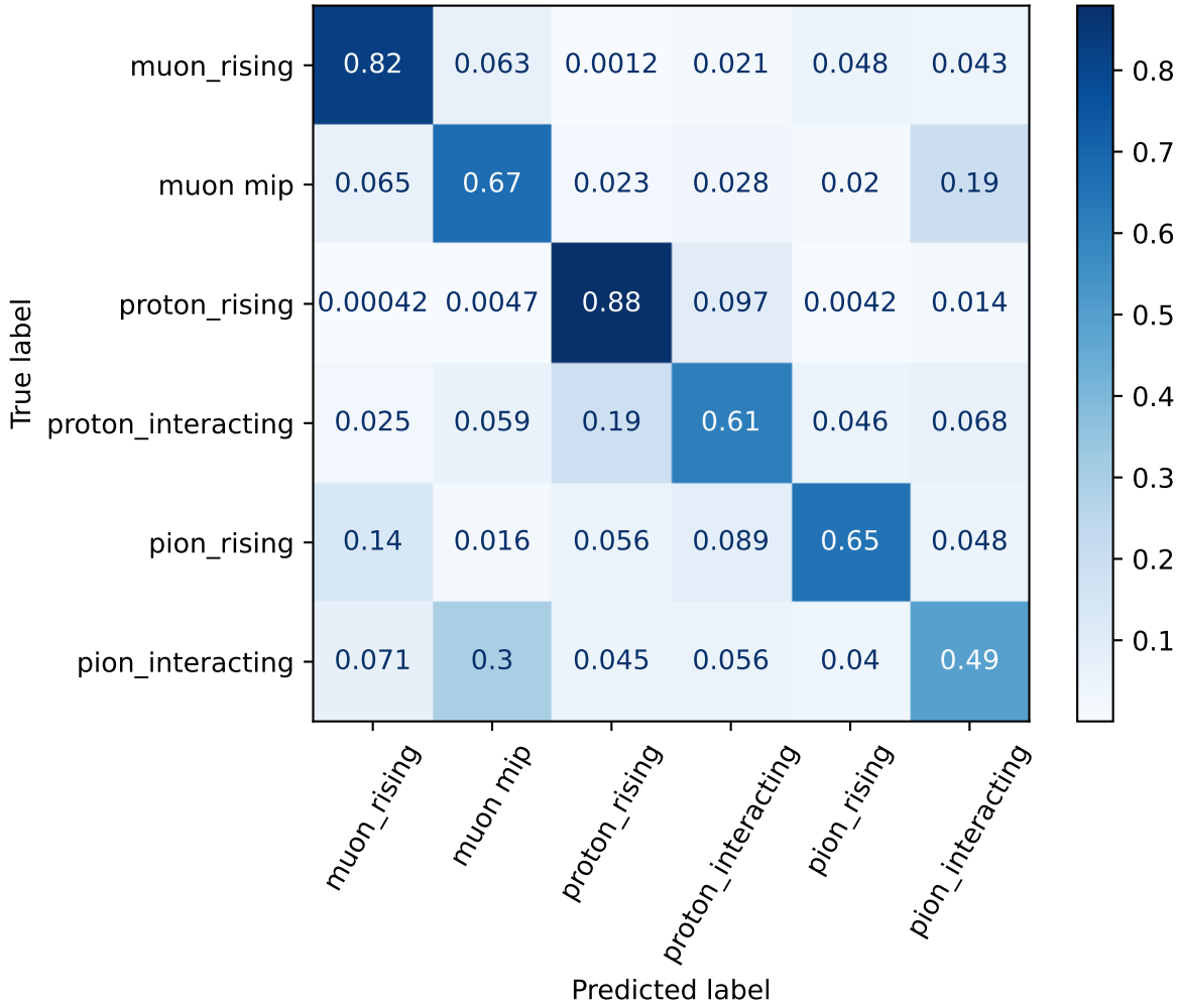
efficiency confusion matrix - learning rate: 0.0075 max depth: 5 subsample frac: 0.5
