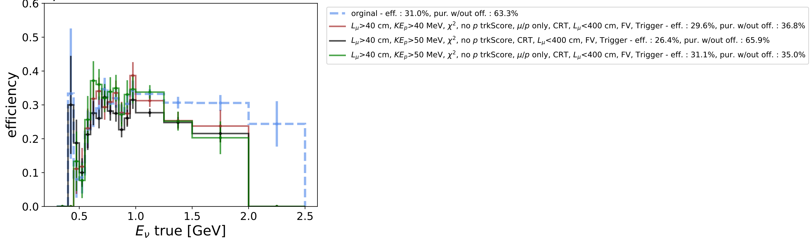
1\mu Np slices - ICARUS RUN 4 - 1.20 \times 10^{20} POT
