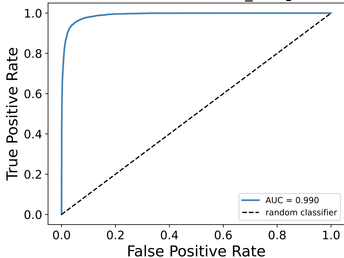
ROC curve — muon_rising
