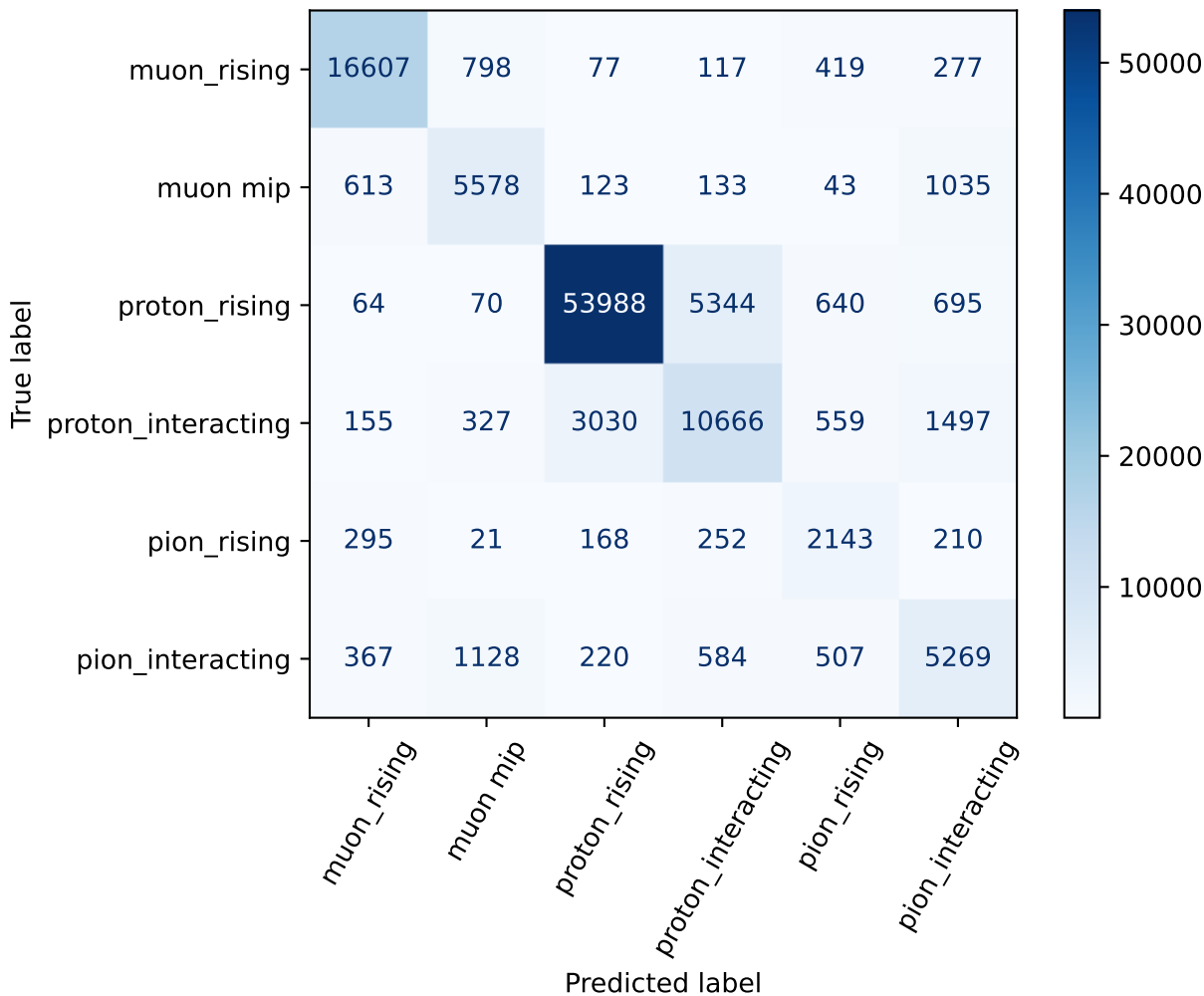
confusion matrix - 70% stat train ONLY COLL - test ALL PLANES
