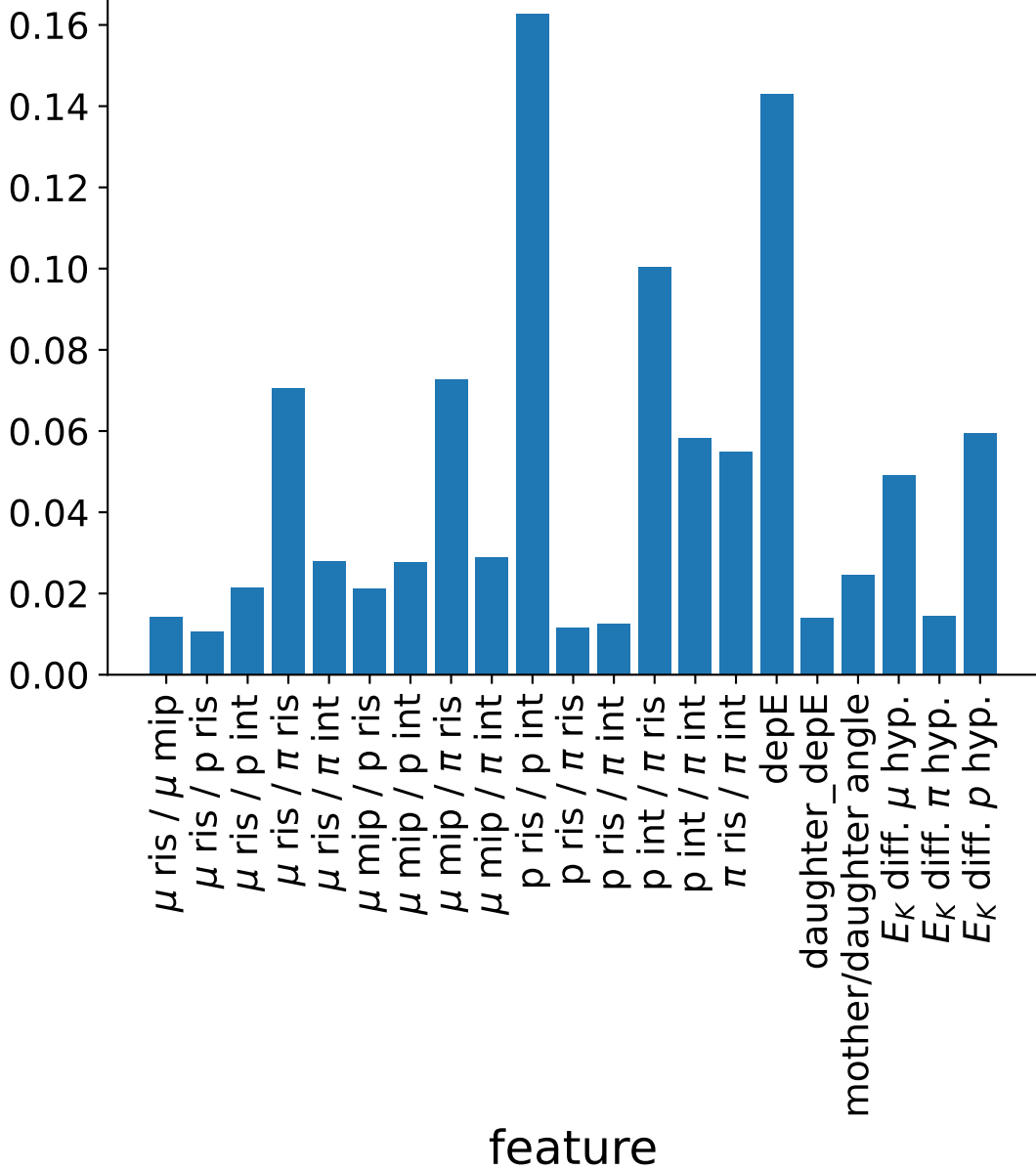
feature importance
