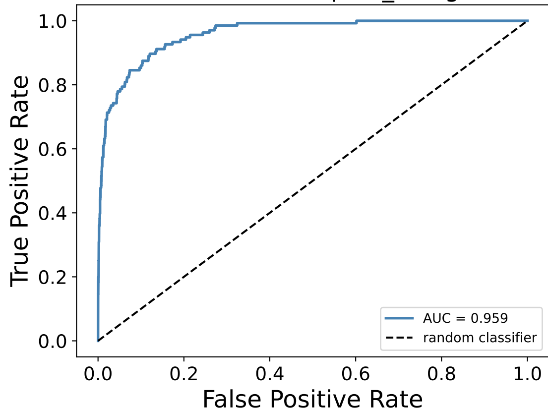
ROC curve — pion_rising
