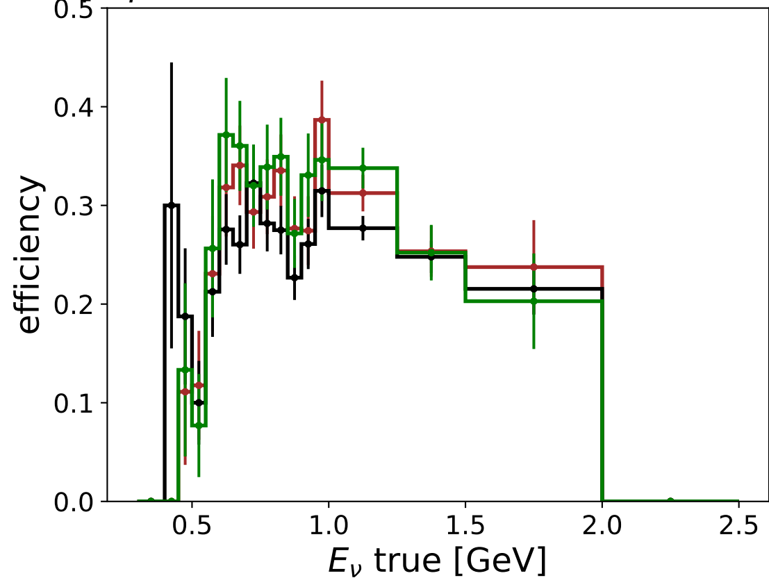
1\mu Np slices - ICARUS RUN 4 - 1.20 \times 10^{20} POT
