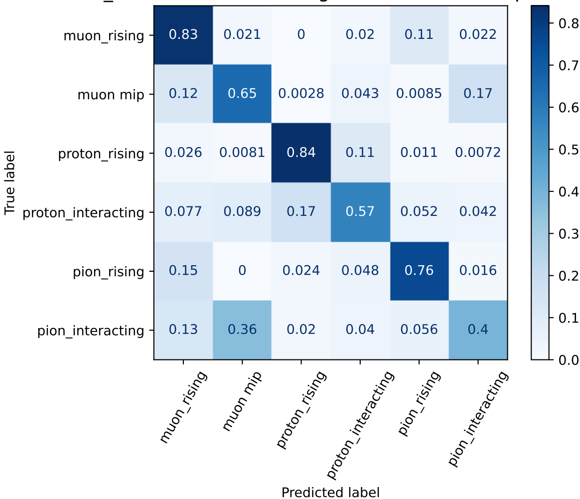
AdaBoost_efficiency confusion matrix n_estimators: 60 learning rate: 0.005 max depth: 5
